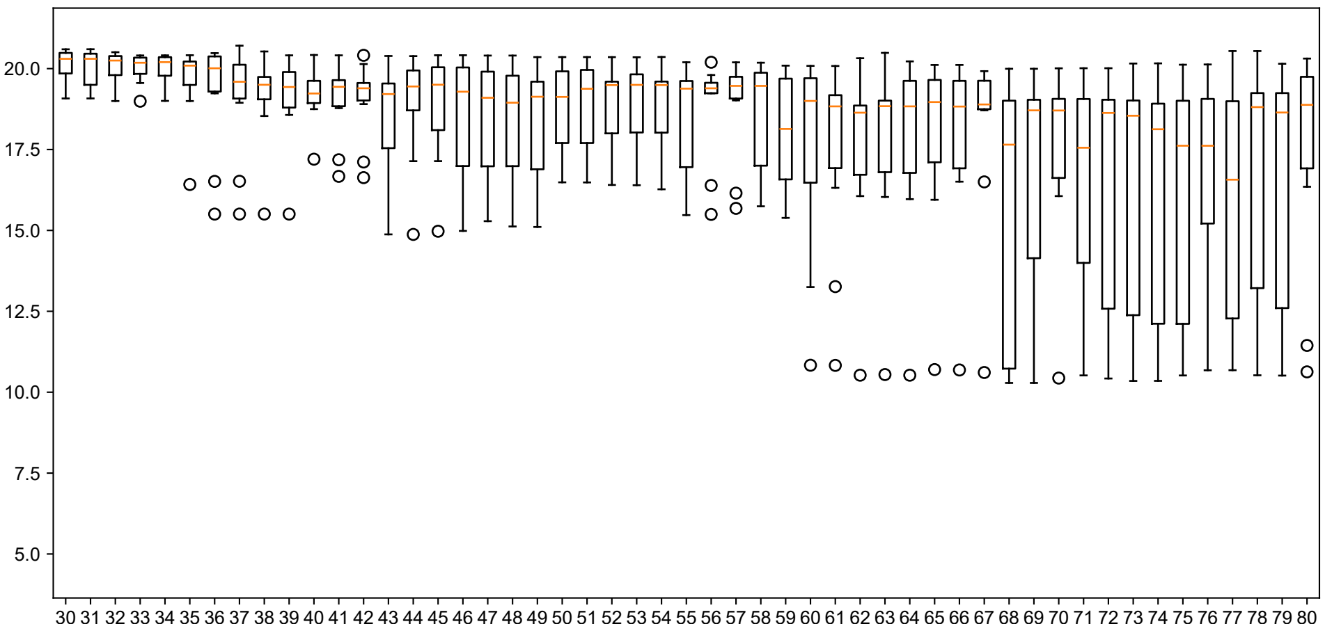
rf
