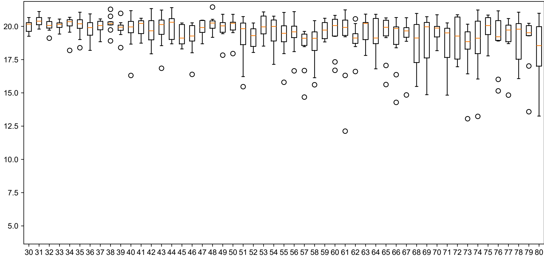
mutual_info_classif
