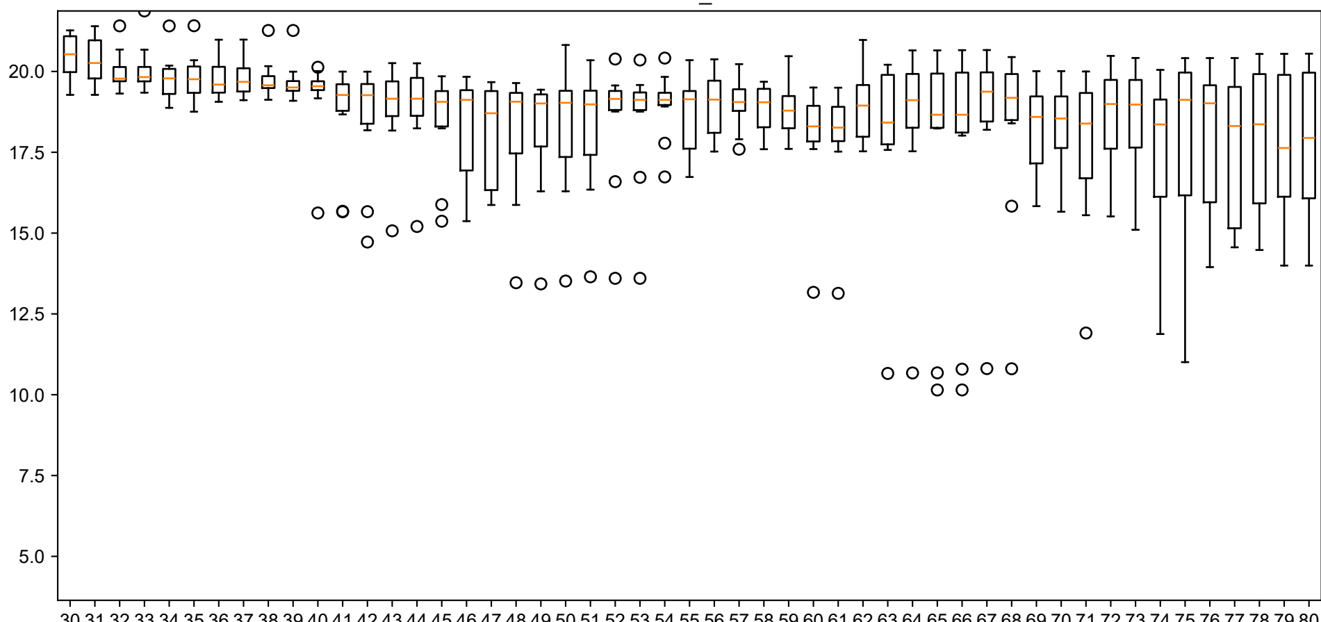
xgb
